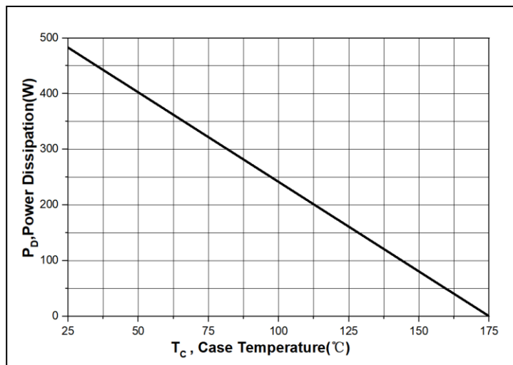
Figure8. Power Dissipation vs. Case Temperature
