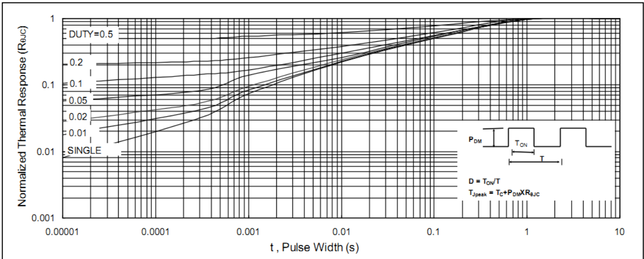
Figure 9: Transient Thermal Impedance
