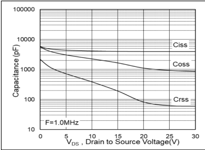
Figure 7: Capacitance
