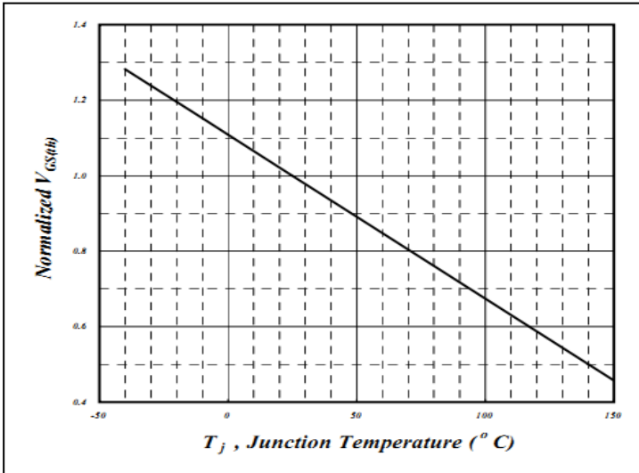
Figure 3: Gate Threshold Voltage Vs. Junction Temperature
