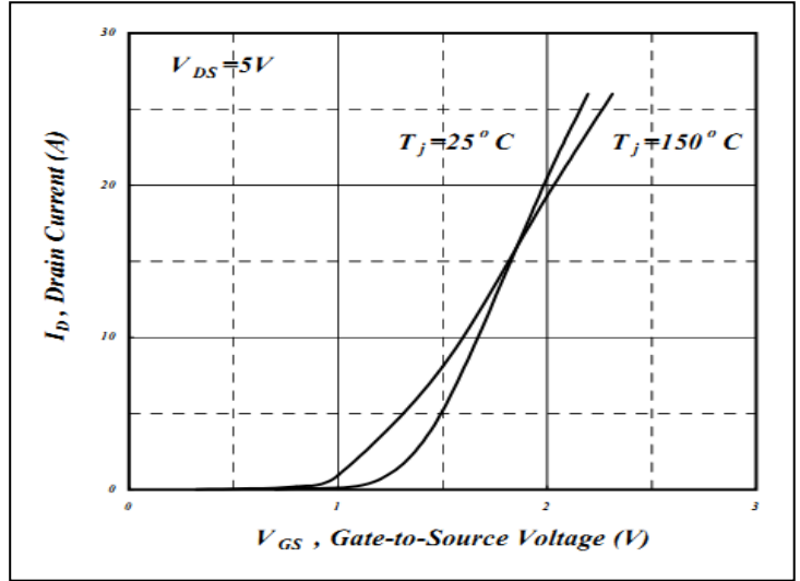
Figure 8: Transfer Characteristics
