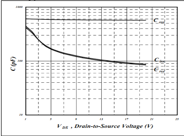
Figure 7: Capacitance Characteristics
