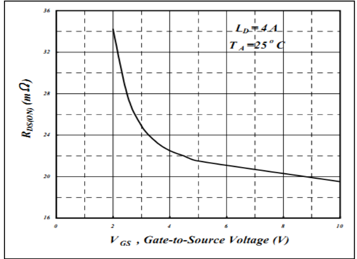
Figure 2: On-Resistance Vs. Gate Voltage
