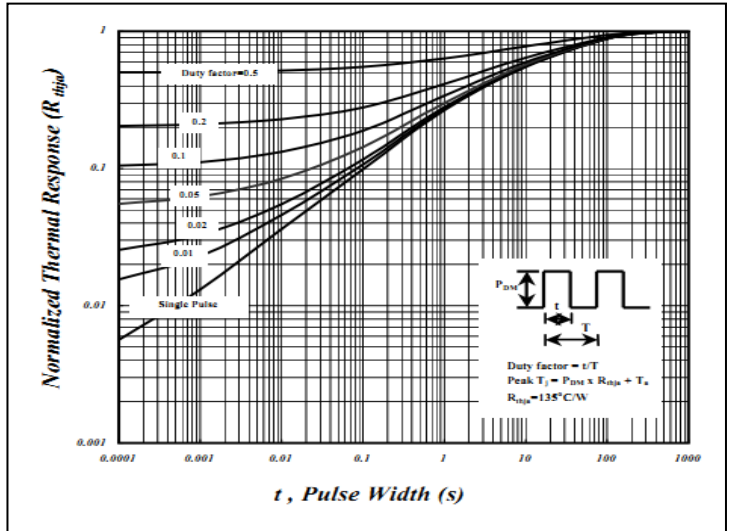
Figure 10: Maximum Effective Transient Thermal Impedance, Junction-to-Case
