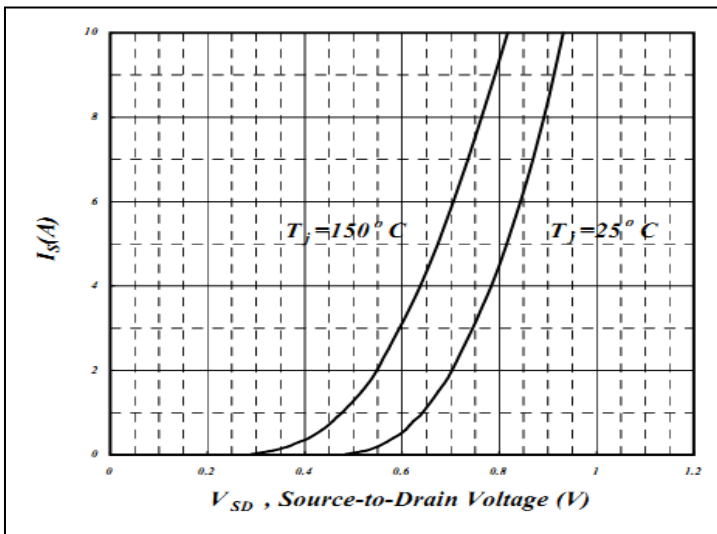
Figure 5: Forward Characteristics Of Reverse Diode
