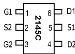
Marking and Pin Assignments
