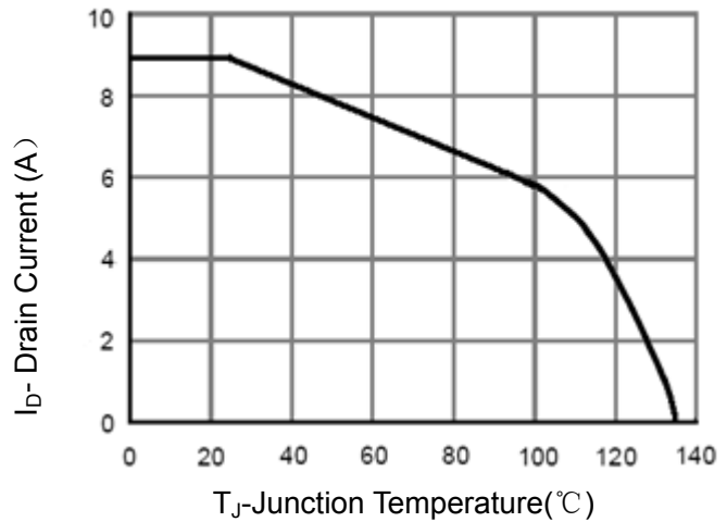
Figure 4 Drain Current
