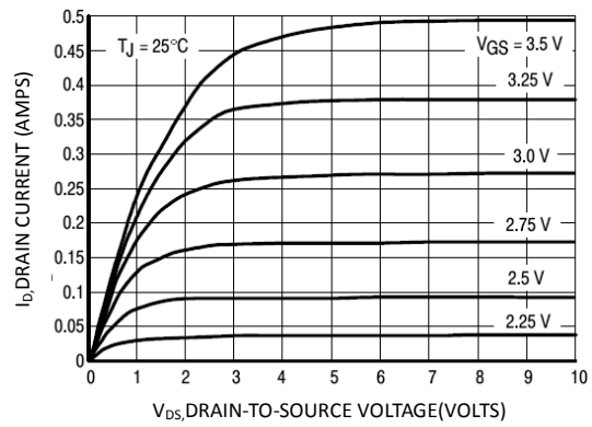
Fig 2: Output Curve
