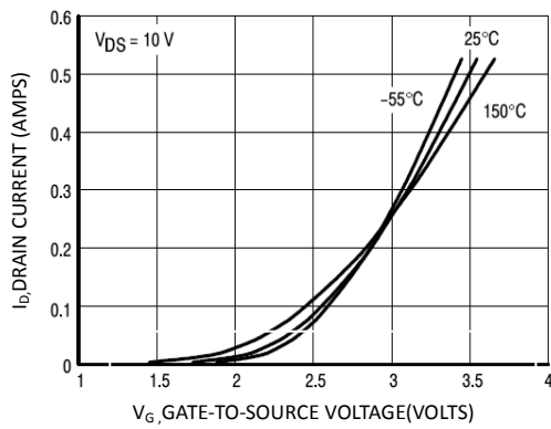
Fig 1: Transfer Characteristics
